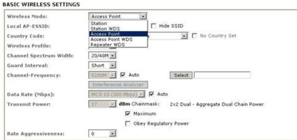
Fig Basic Wireless Settings (Access Point/ Access Point WDS)
